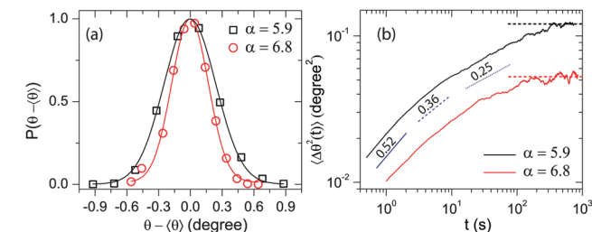
Fig. 5 (a) Probability distribution of angular fluctuations of the rod, P(\theta - \langle \theta \rangle) , for two rods of different aspect ratio, \alpha . The distributions for both rods peak at (\theta - \langle \theta \rangle) \sim 0 . The probability axis has been scaled such that P(\theta - \langle \theta \rangle) = 1 at (\theta - \langle \theta \rangle) = 0 . Solid lines are Gaussian fits to the data. (b) Angular mean-squared displacement \langle \Delta\theta^2(t) \rangle for the two rods whose distributions are shown in (a). The solid, dashed, and dotted blue line segments have slopes of 0.52, 0.36 and 0.25, respectively. The horizontal dashed lines indicate the saturation value of \langle \Delta\theta^2(t) \rangle .
